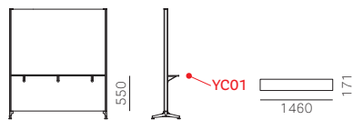
Item YC01_L150
